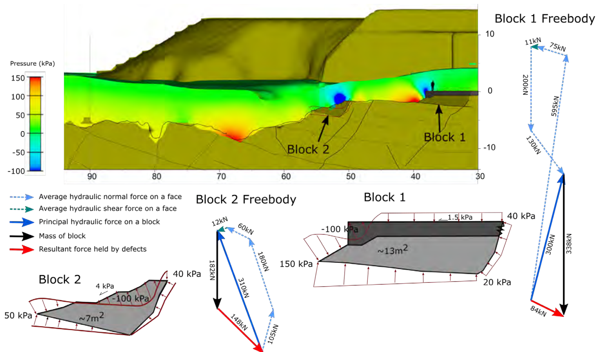
Figure 16: Example of kinematic analysis of selected blocks
