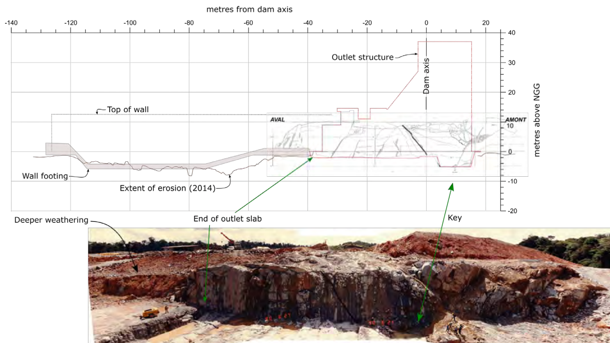
Figure 13: Previous mapping and photographs of geology – right wall of outlet
