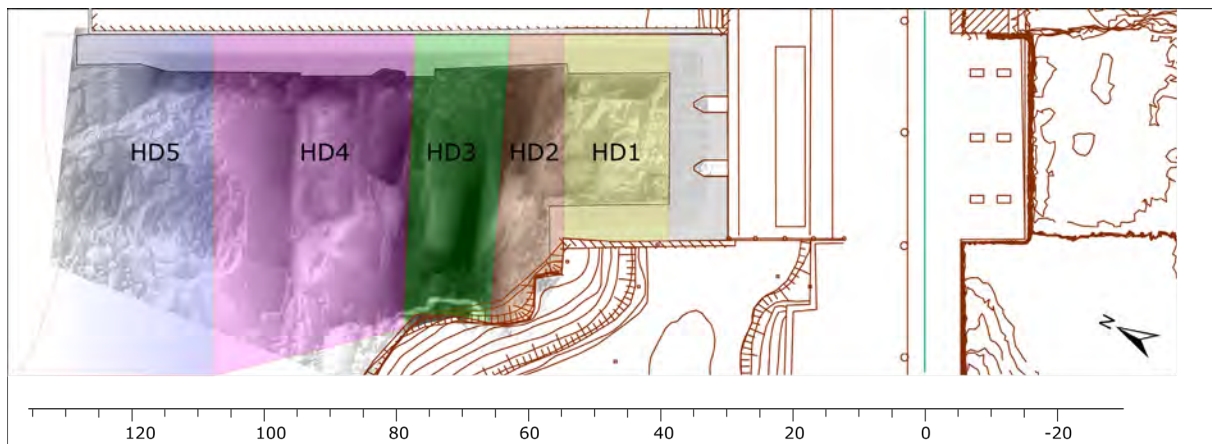
Figure 11: Interpreted hydraulic domains
