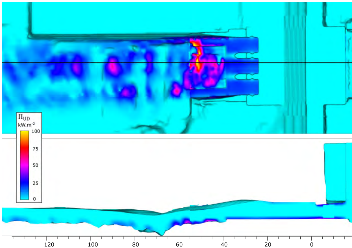
Figure 10: \Pi_{UD} as product of shear stress and velocity (Scenario 4)
