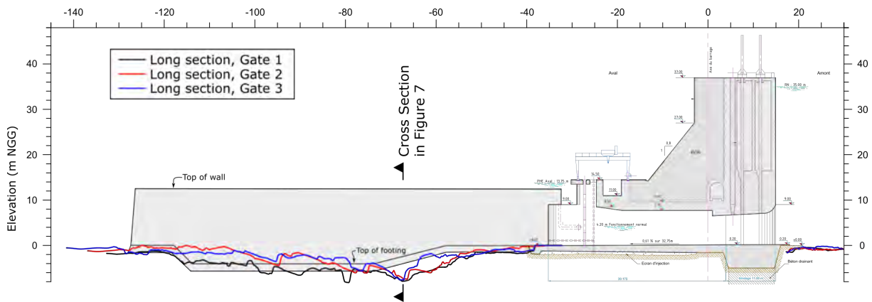
Figure 6: Long section through bottom outlet, 2014 elevation
