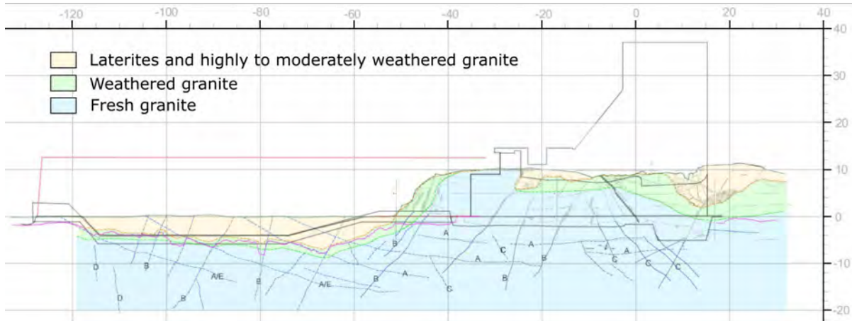
Figure 14: Example of interpreted stratigraphy
