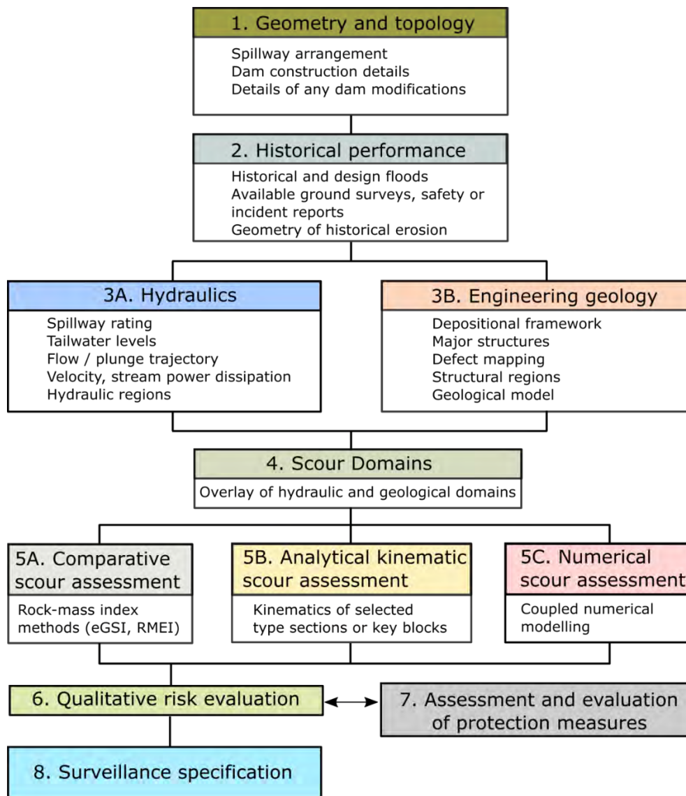
Figure 1: Flow chart for a “hydro-geotechnical scour assessment”
